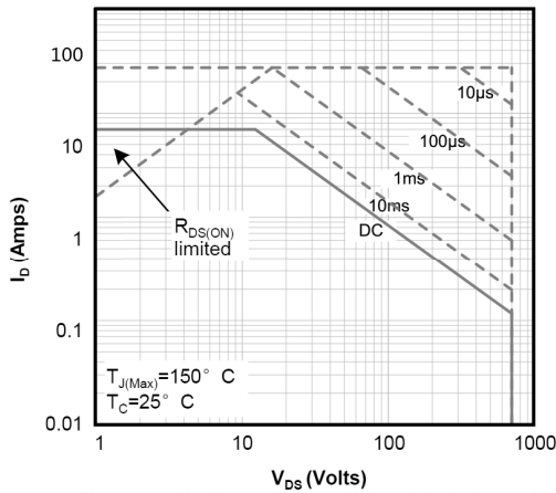
Figure 9 : Maximum Forward Biased Safe Operating Area
